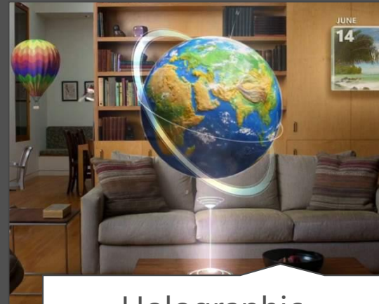
Holographic Computing
